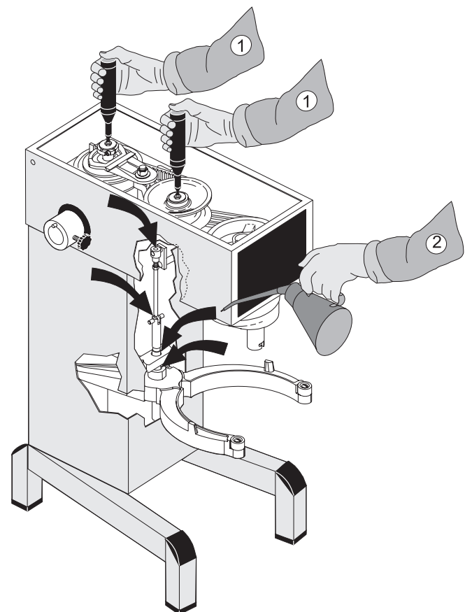
fig.5 Greasing of infinitely variable gear and other movable parts:
