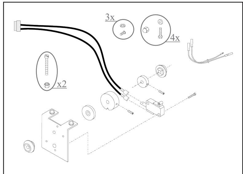
56PG20-39ZB Hardware kit 20L
