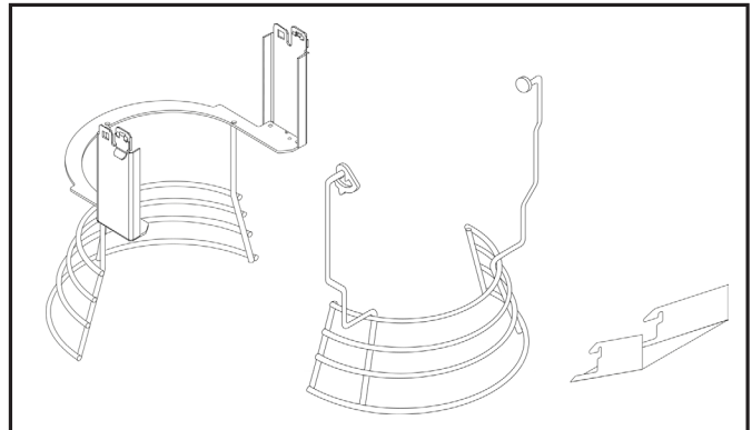
56AG20ZB Removeable grid guard 20L
